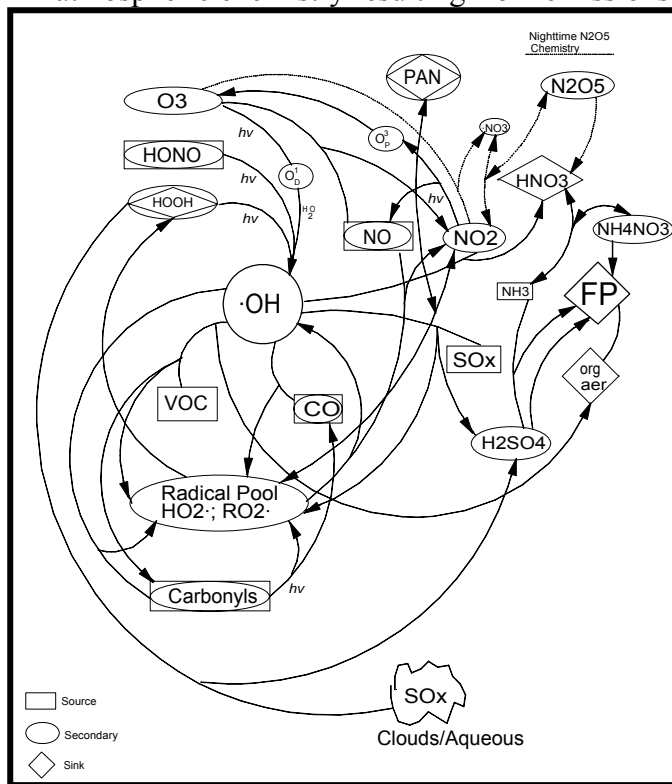
Figure 32. Spaghetti diagram depiction of key atmospheric chemistry pathways responsible for ozone and secondary aerosol formation.
