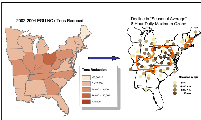
Figure 26. Association between ozone season power plant NO x emission reductions and observed ozone for from 2002-2004. An average 1.1%/year rate of decline in ozone between 1997 and 2002 increased to 3.1%/year between 2002 and 2004, the period associated with deployment of NO x SIP CALL reductions (EPA, 2005).
