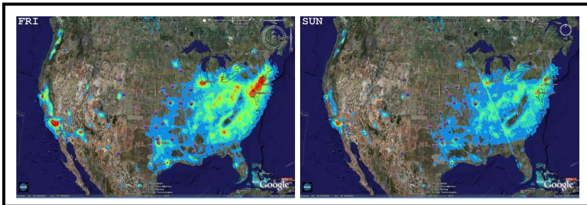
Figure 21. 2004 OMI NO 2 column images aggregated for all Fridays (left) and Sundays (right) indicating weekend/weekday patterns associated with reduced Sunday emissions (source, Husar).
